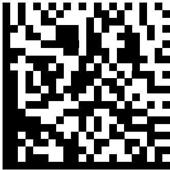
Cancel Dialog
